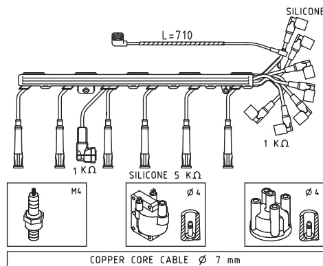
COPPER CORE CABLE Ø 7 mm
