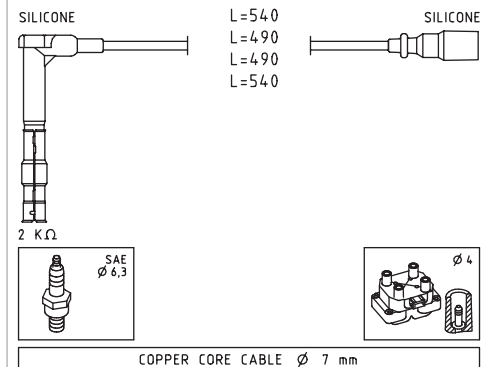
COPPER CORE CABLE Ø 7 mm
