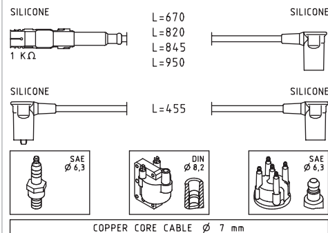
COPPER CORE CABLE Ø 7 mm
