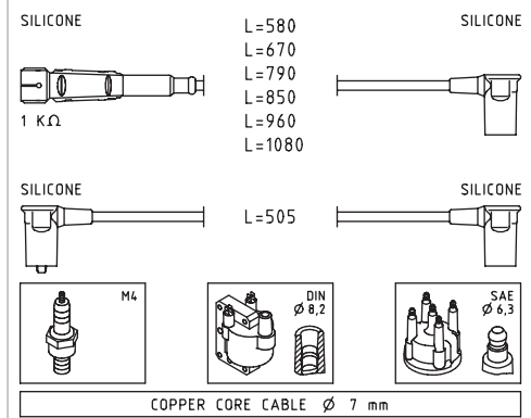
COPPER CORE CABLE Ø 7 mm
