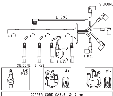
COPPER CORE CABLE Ø 7 mm
